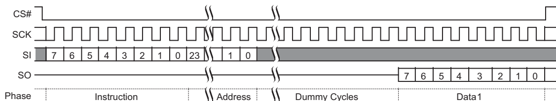
Figure 52. RSFDP Command Sequence
