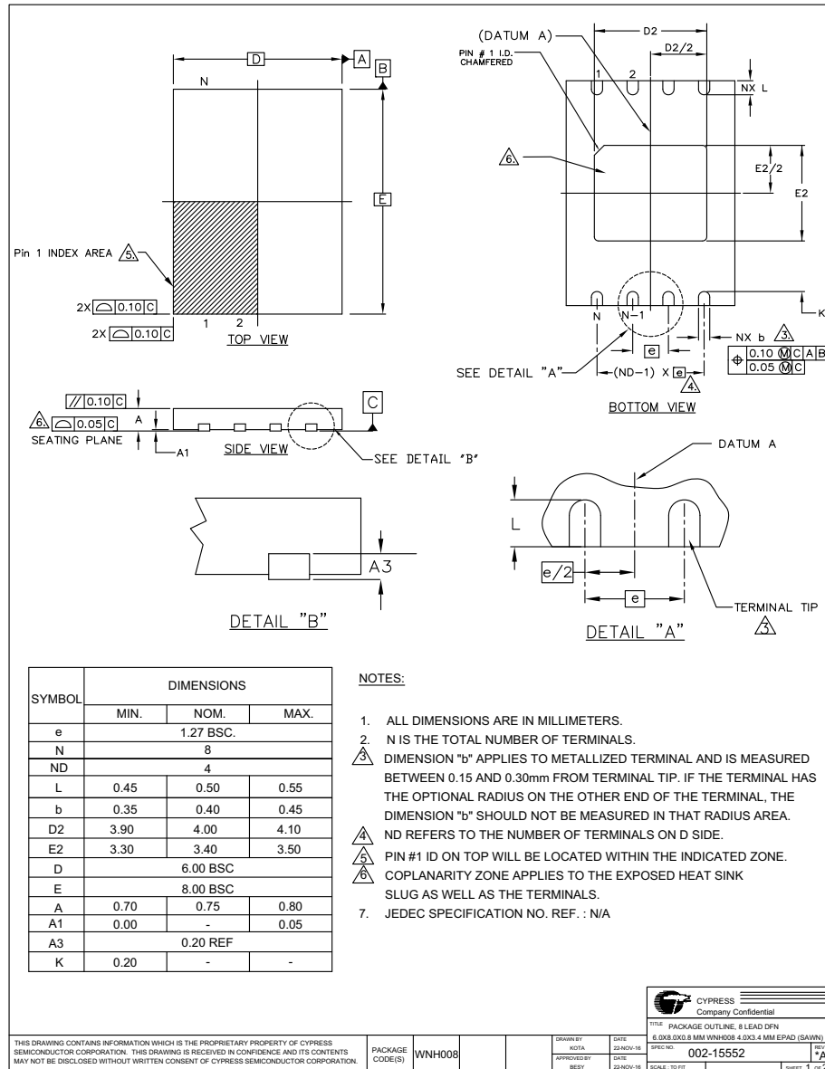
Figure 41. WSON 8-Contact 6x8 mm Leadless (WNH008)
