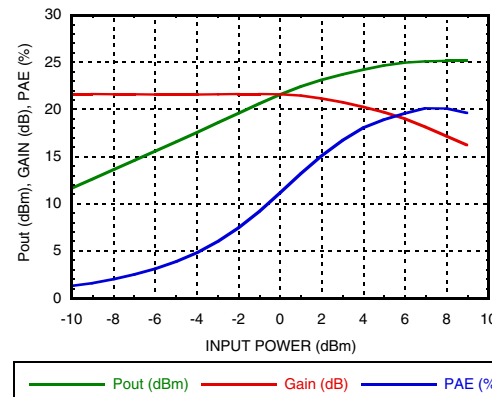
Power Compression @ 24 GHz
