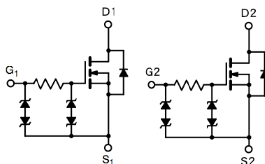
Dual N-Channel MOSFET
