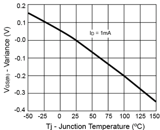
Threshold Voltage
