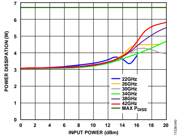
Figure 38. Power Dissipation (P DISS ) vs. Input Power, T A = 85°C
