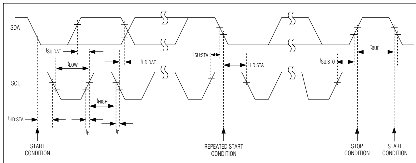
Figure 6. Serial Interface Timing
