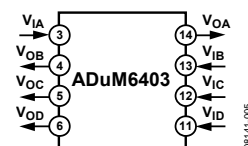
Figure 5. ADuM6403
