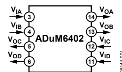
Figure 4. ADuM6402
