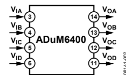
Figure 2. ADuM6400
