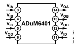
Figure 3. ADuM6401
