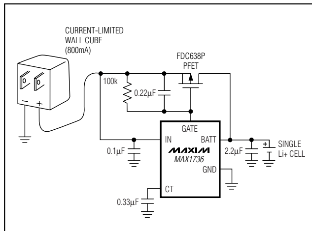
Figure 3. Simple Application Circuit
