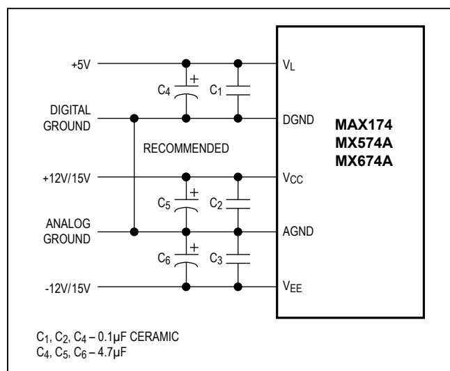
Figure 9. Power-Supply Bypassing
