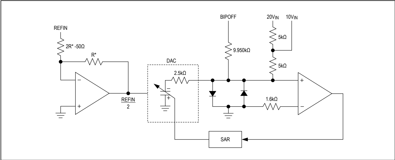
Figure 3. Analog Equivalent Circuit
