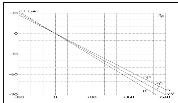
Figure 8. Gain vs. Control Voltage ( E_C ) with Temp ( ^{\circ}\text{C} )
