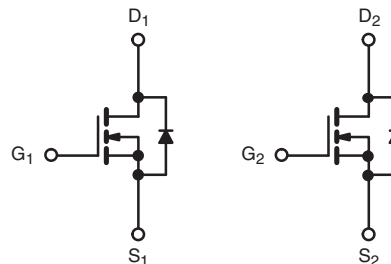
N-Channel MOSFET
