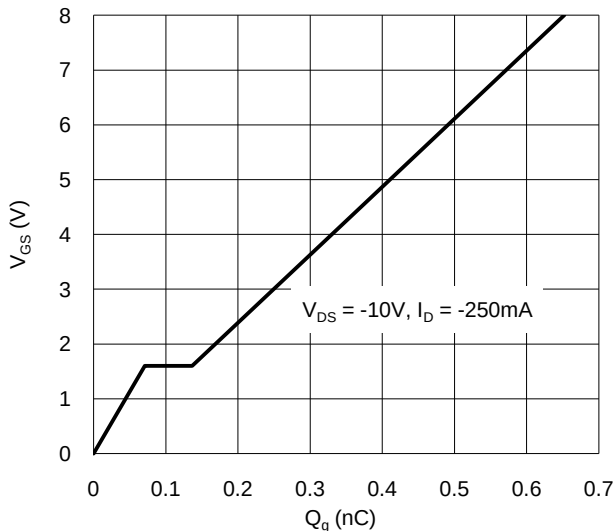
Figure 23. Gate Charge
