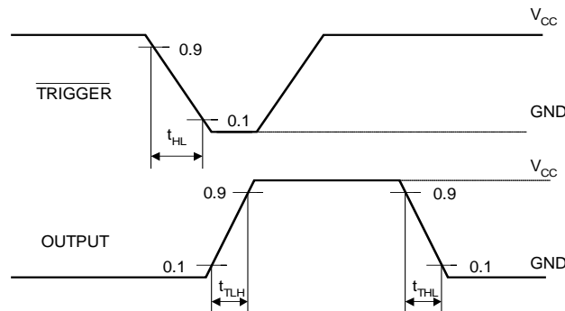
Figura 2. Switching Waveforms
