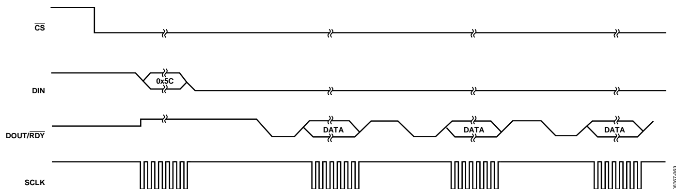
Figure 27. Continuous Read
