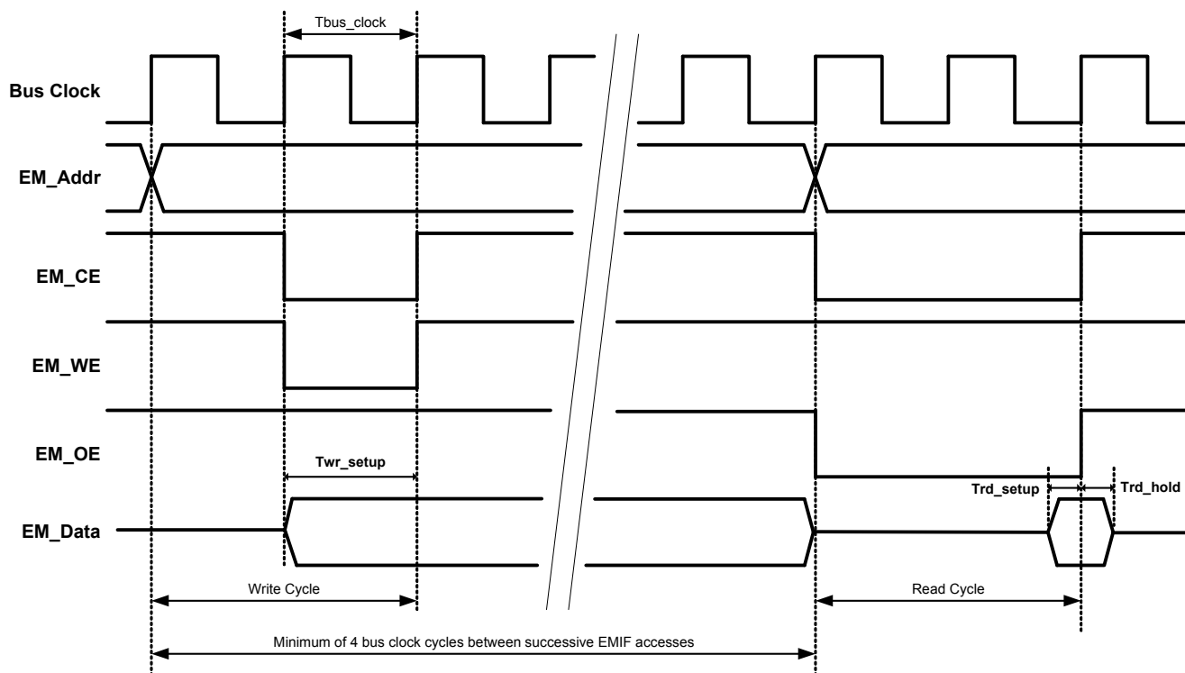
Figure 11-66. Asynchronous Write and Read Cycle Timing, No Wait States
