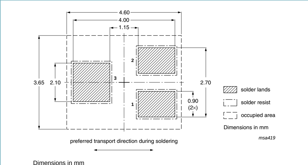
Fig 22. Wave soldering footprint SOT323 (SC-70)
