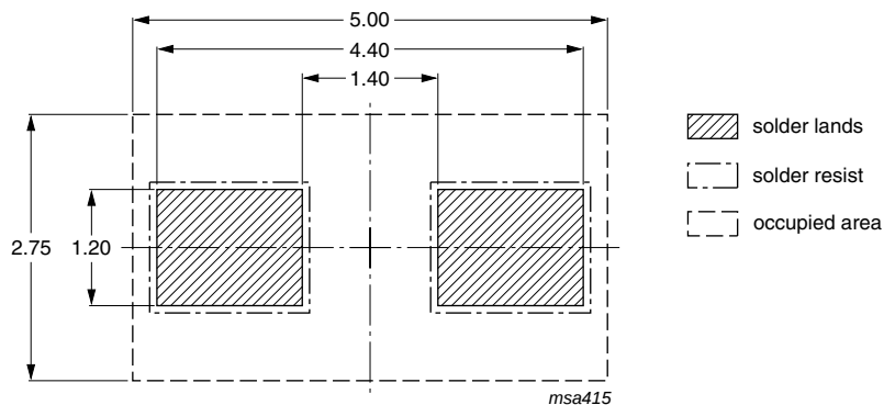
Fig 14. Reflow soldering footprint SOD323 (SC-76)
