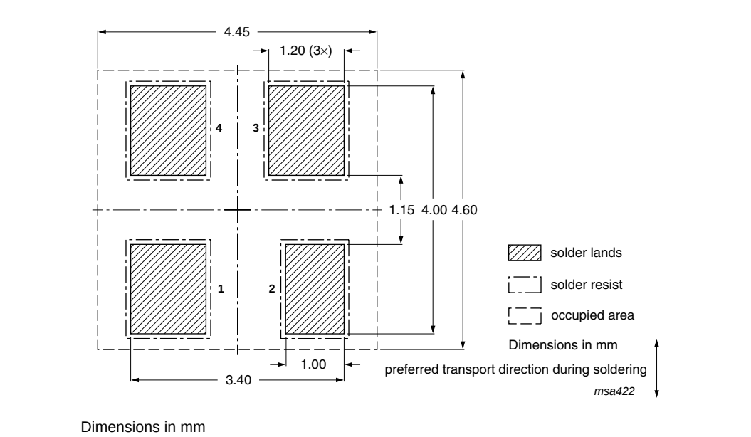
Fig 24. Wave soldering footprint SOT143B
