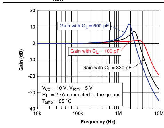
Figure 20. Frequency response for different capacitive load at V_{CC} = 10 V, V_{icm} = 5 V and T = 25 °C
