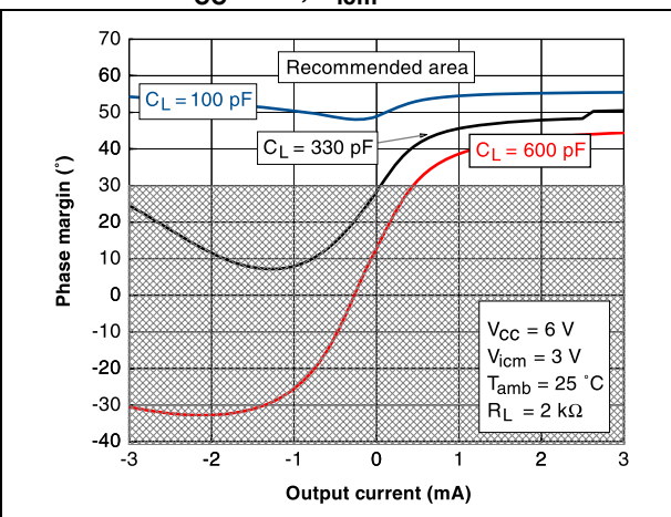
Figure 25. Phase margin vs. output current, at V_{CC} = 6 V, V_{icm} = 3 V and T = 25 °C
