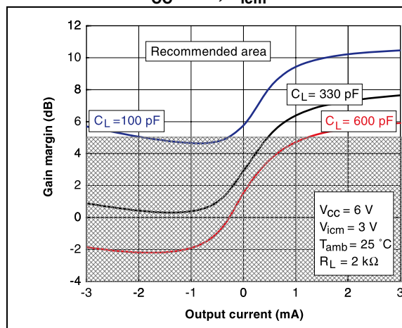
Figure 22. Gain margin vs. output current, at V_{CC} = 6 V, V_{icm} = 3 V and T = 25 °C
