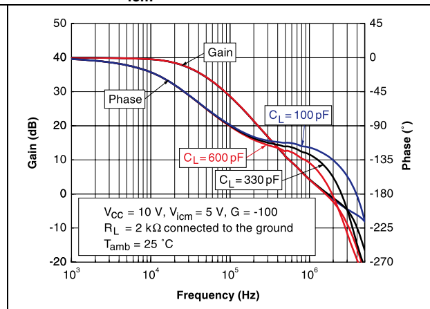
Figure 17. Voltage gain and phase for different capacitive load at V_{CC} = 10\text{ V} , V_{icm} = 5\text{ V} and T = 25\text{ °C}
