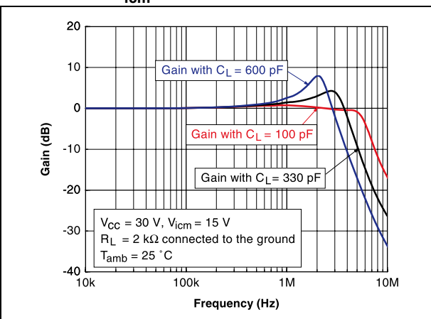
Figure 21. Frequency response for different capacitive load at V_{CC} = 30 V, V_{icm} = 15 V and T = 25 °C
