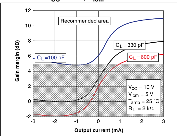
Figure 23. Gain margin vs. output current, at V_{CC} = 10 V, V_{icm} = 5 V and T = 25 °C
