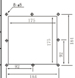
PANEL CUTOUT
