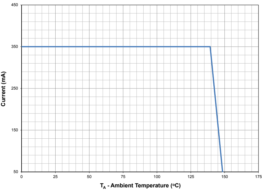
Figure 11. Maximum forward current vs. ambient temperature, based on T_{JMAX} = 150^{\circ}\text{C} for Automotive White.
