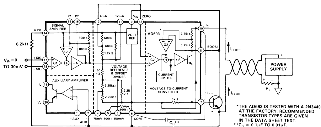
Figure 11. Using an External Pass Transistor to Minimize Self-Heating Errors
