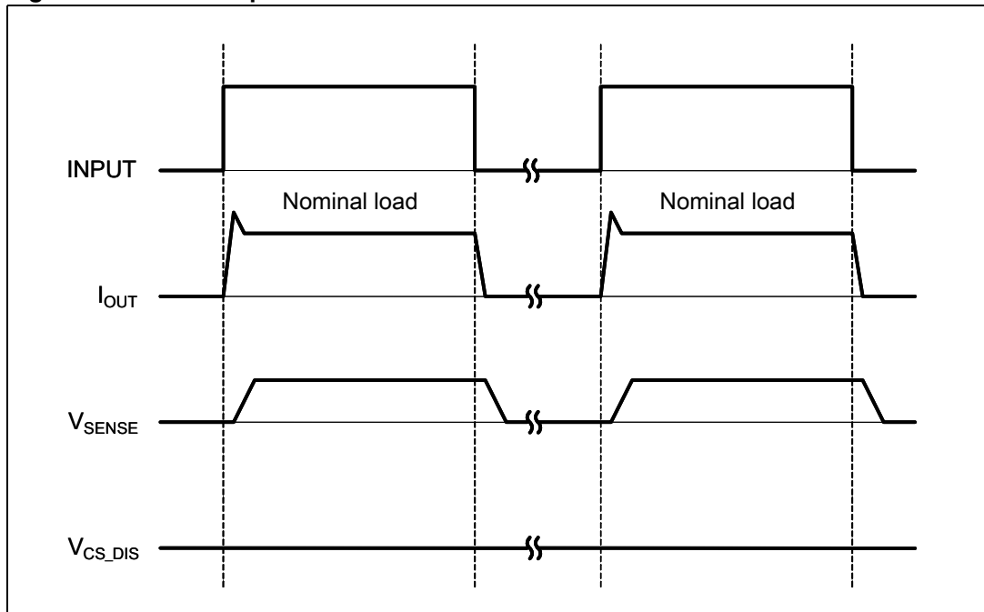
Figure 10. Normal operation
