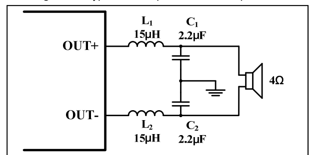
Figure 15 Typical LC Output Filter for 4Ω Speaker
