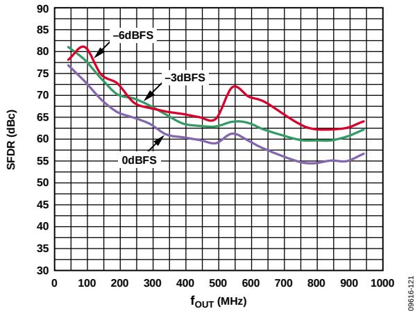
Figure 21. SFDR vs. f_{\text{OUT}} over Digital Full Scale
