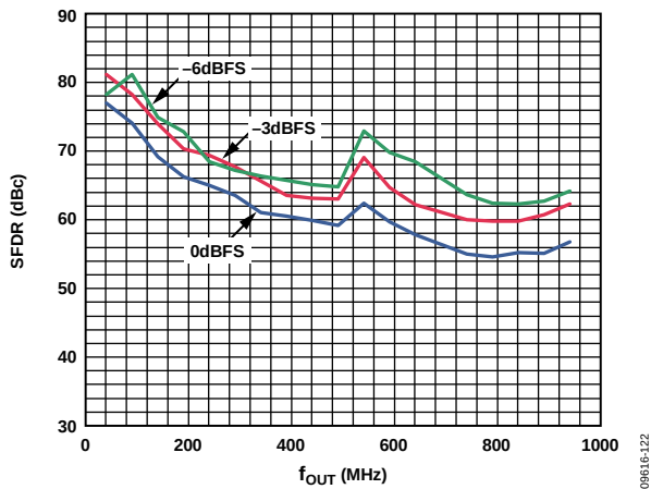
Figure 22. SFDR for Second Harmonic vs. f_{\text{OUT}} over Digital Full Scale
