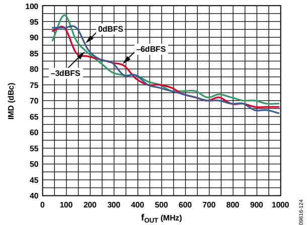
Figure 24. IMD vs. f_{\text{OUT}} over Digital Full Scale
