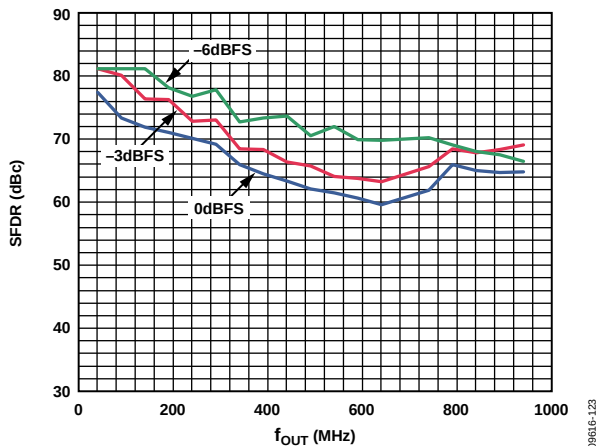
Figure 23. SFDR for Third Harmonic vs. f_{\text{OUT}} over Digital Full Scale
