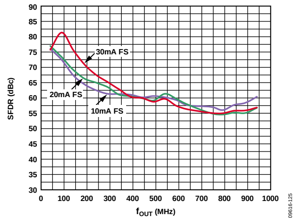
Figure 25. SFDR vs. f_{\text{OUT}} over DAC I_{\text{OUTFS}}
