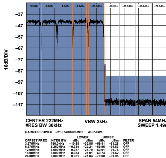
Figure 131. Low Band Narrow-Band ACLR (Worse Side)
