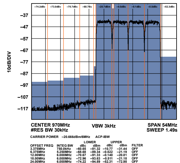
Figure 127. High Band Narrow-Band ACLR
