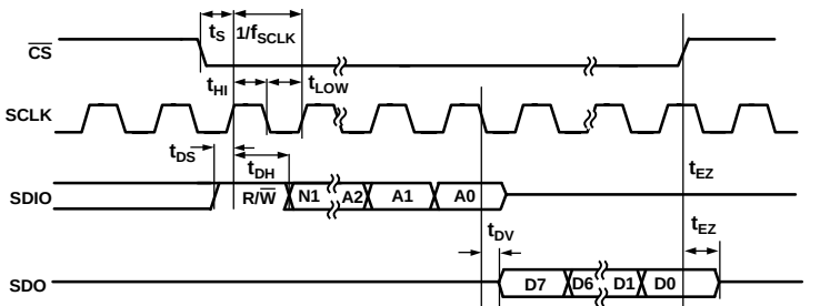
Figure 156. SPI 4-Wire Read Operation Timing
