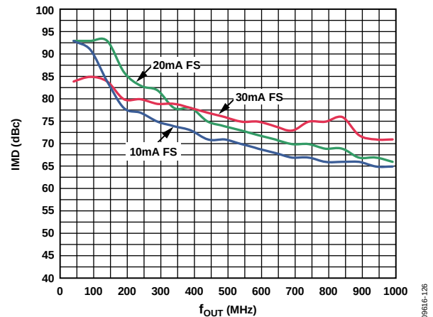
Figure 26. IMD vs. f_{\text{OUT}} over DAC I_{\text{OUTFS}}
