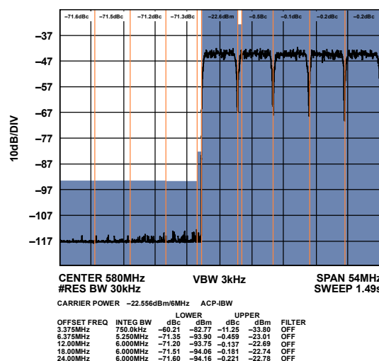
Figure 132. Mid Band Narrow-Band ACLR (Worse Side)
