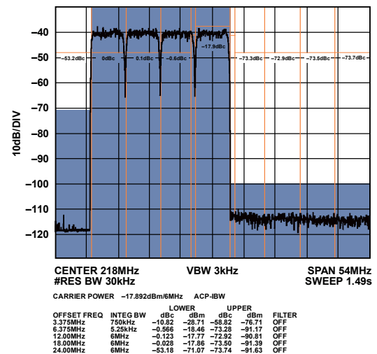
Figure 51. Low Band Narrow-Band ACLR (Worse Side)
