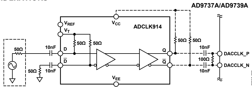
Figure 173. ADCLK914 Interface to the AD9737A/AD9739A CLK Input
