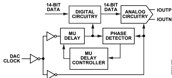
Figure 165. AD9737A Mu Delay Controller Block Diagram
