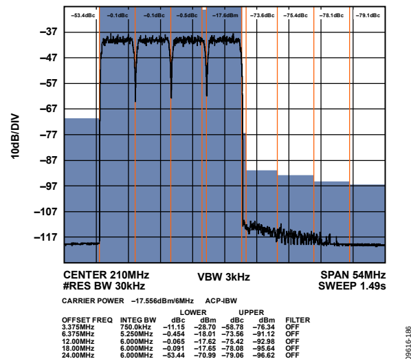
Figure 125. Low Band Narrow-Band ACLR (Worse Side)
