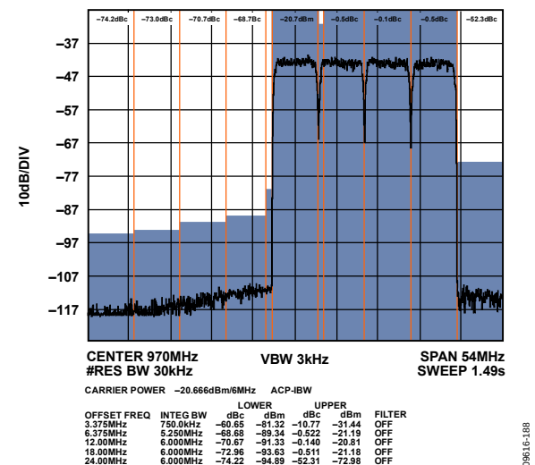
Figure 127. High Band Narrow-Band ACLR
