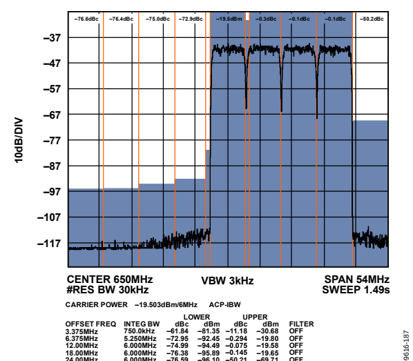
Figure 126. Mid Band Narrow-Band ACLR (Worse Side)
