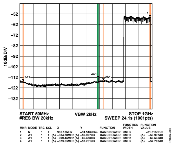
Figure 142. High Band Wideband ACLR
