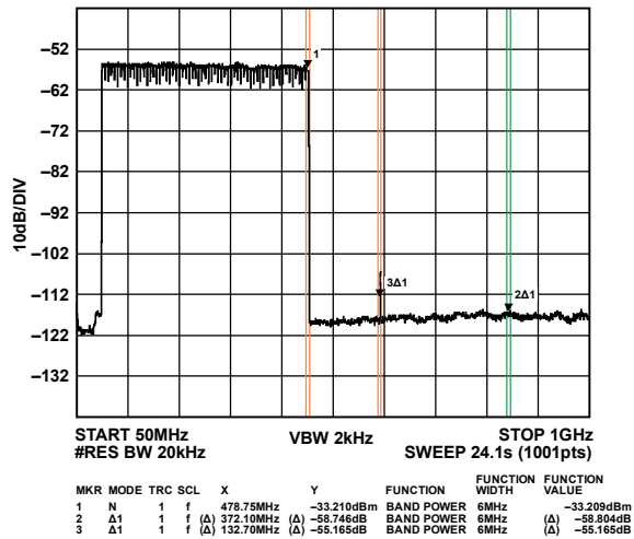
Figure 146. 64-Carrier Low Band Wideband ACLR
