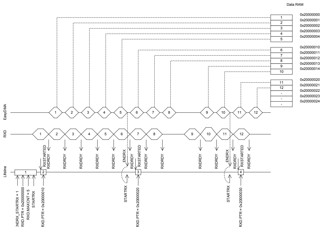
Figure 95: UARTE reception
