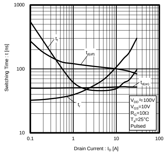
Fig.10 Switching Characteristics
