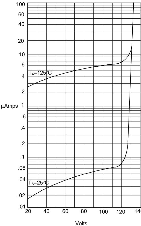
Figure 7 Typical Reverse Characteristics
