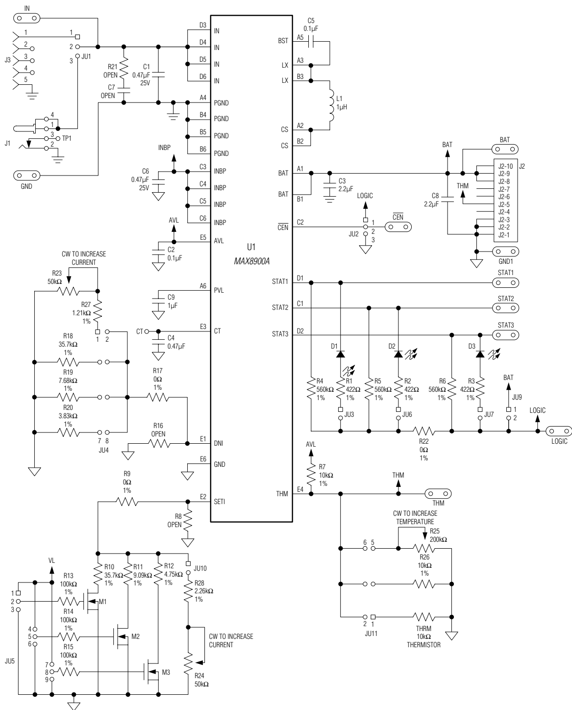
Figure 9. MAX8900A EV Kit Schematic
