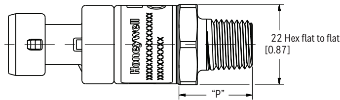
Figure 6. Pressure Port Type Dimensions (For reference only: mm/[in.]) 1
