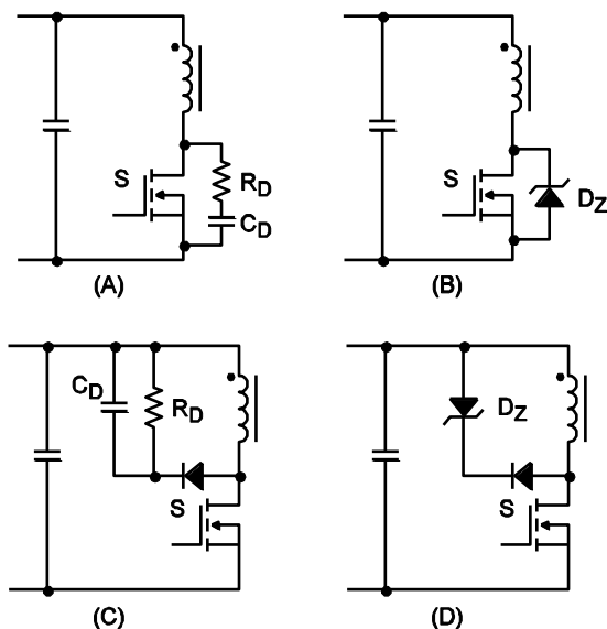
Figure 5—Snubber Designs
