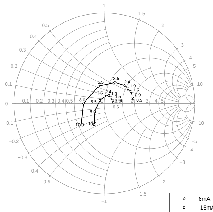
Figure 5-16 Source Impedance for Minimum Noise Figure Z_{opt} = f(f) , V_{CE} = 3\text{ V} , I_C = 6 / 15\text{ mA}
