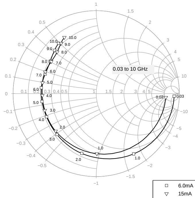
Figure 5-15 Input Matching S_{11} = f(f) , V_{CE} = 3\text{ V} , I_C = 6 / 15\text{ mA}
