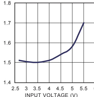
Current Limit vs. Input Voltage
