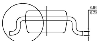
SIDE VIEW-1
