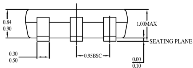
SIDE VIEW - 2
