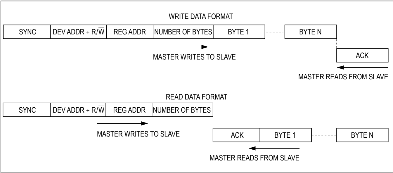
Figure 22. GMSL-UART Protocol for Base Mode
