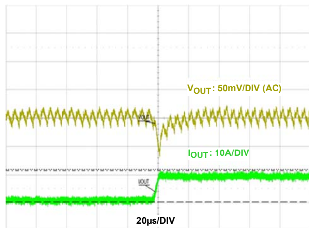
FIGURE 14. TRANSIENT RESPONSE 2A/μs
