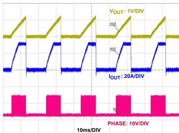
FIGURE 12. HICCUP OCP
