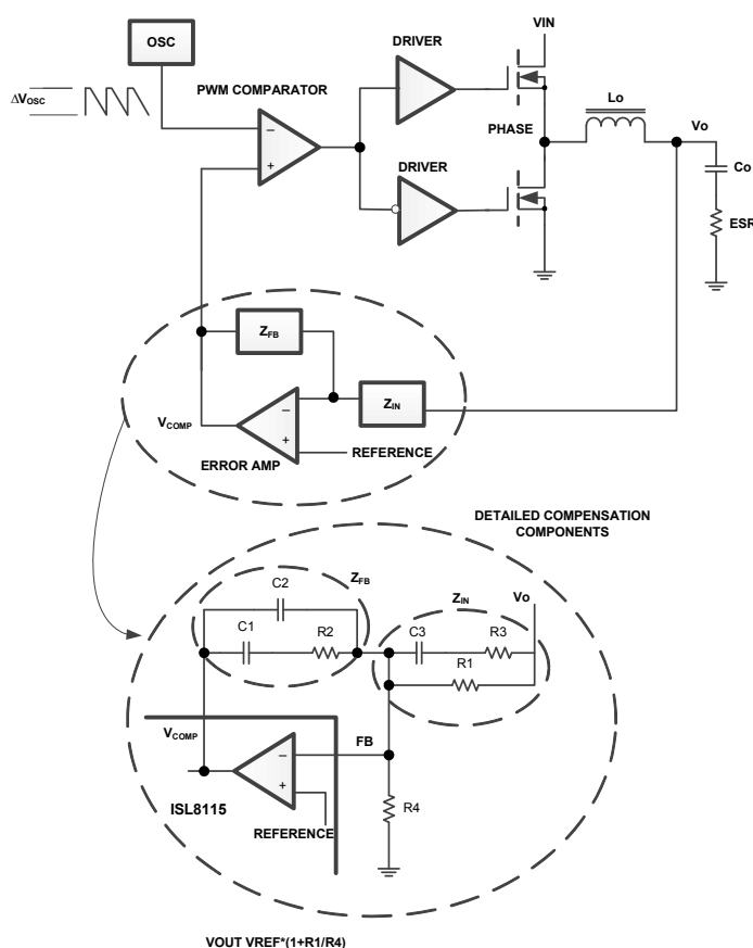
FIGURE 31. VOLTAGE- MODE BUCK CONVERTER COMPENSATION DESIGN
