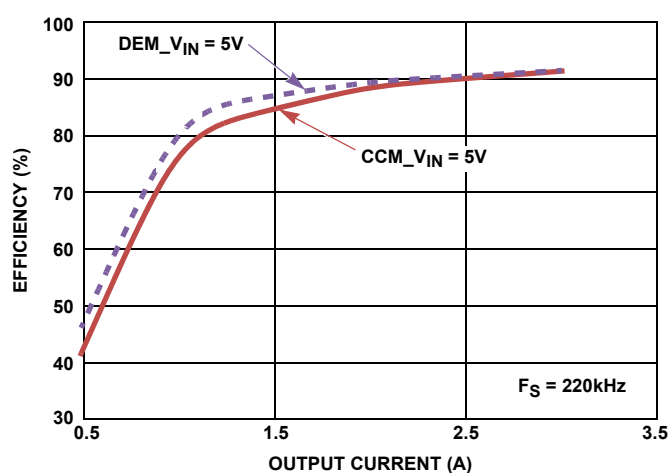
FIGURE 7. EFFICIENCY vs LOAD CURRENT AT 5V INPUT
