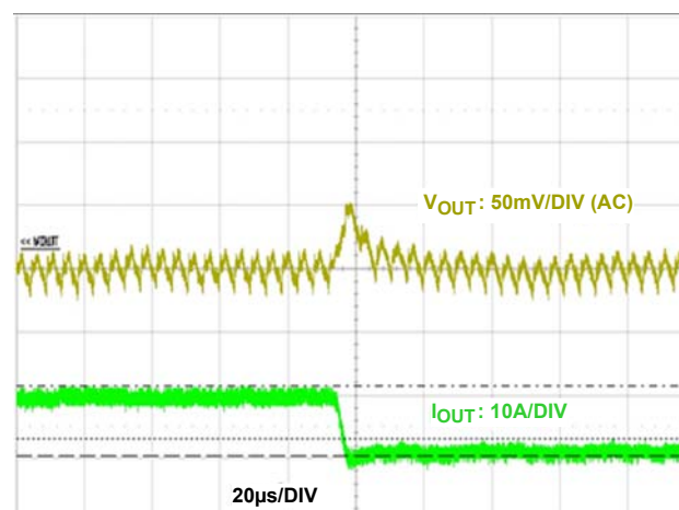
FIGURE 13. TRANSIENT RESPONSE 2A/μs
