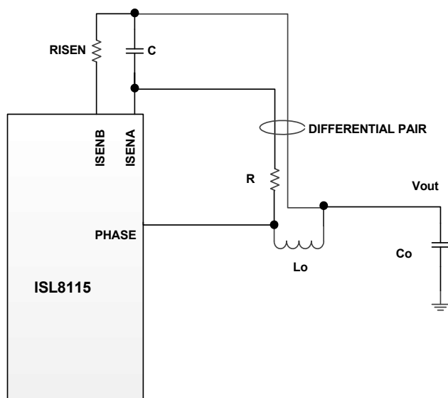
FIGURE 34. CURRENT SENSING LOOP
