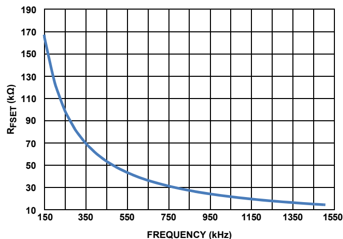
FIGURE 21. FREQUENCY vs R_{FSET}
