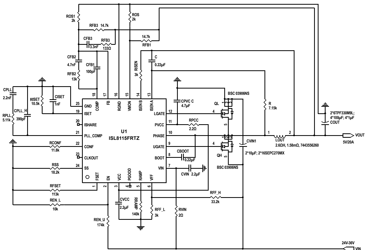
FIGURE 2. TYPICAL APPLICATION CIRCUIT, 24V-36V INPUT, 5V/20A OUTPUT
