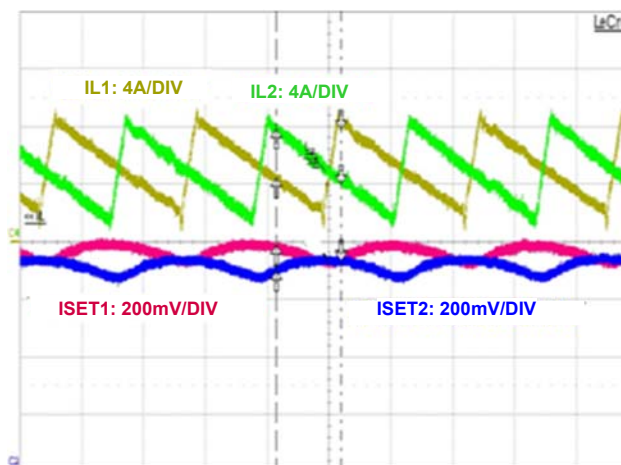
FIGURE 15. CURRENT SHARING WITH 2-PHASE CONFIGURATION
