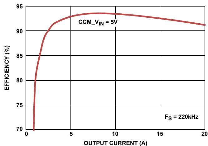
FIGURE 5. EFFICIENCY AT 5V INPUT, 1.5V OUTPUT
