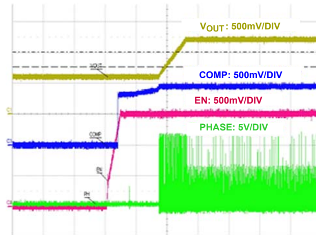
FIGURE 11. PRE-BIAS START-UP
