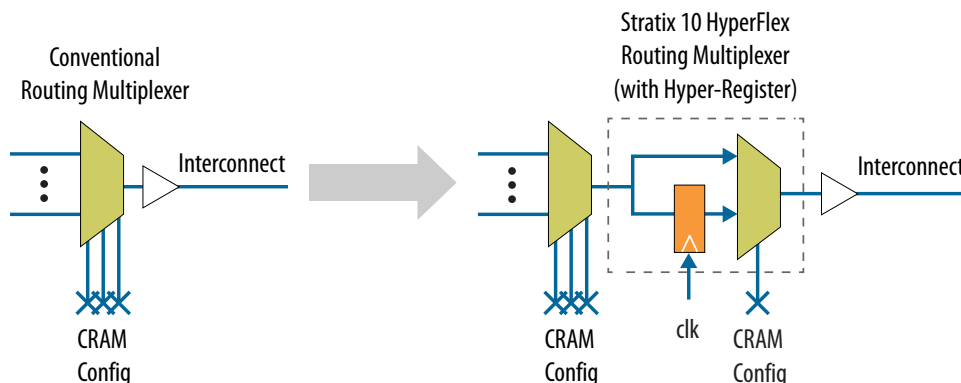
Figure 5. Bypassable Hyper-Register
