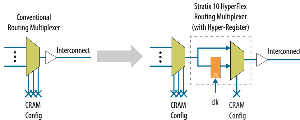
Figure 5. Bypassable Hyper-Register
