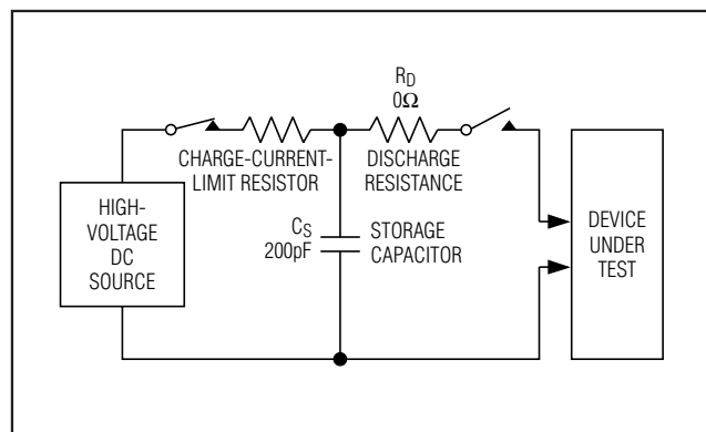
Figure 16. Machine Model ESD Test Circuit
