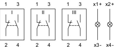
Wiring diagram 3
