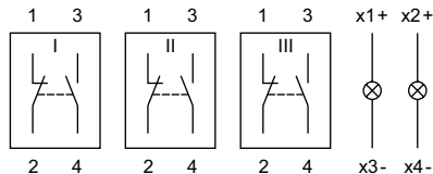
Wiring diagram 5
