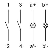
Wiring diagram 9
