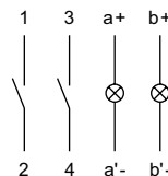
Wiring diagram 10
