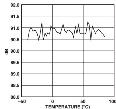
TPC 6. SNR vs. Temperature
