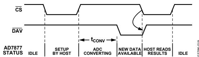
Figure 41. Operation of \overline{DAV} Output
