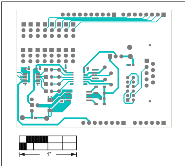
MAX33250E Shield—Top
