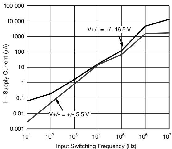
Negative Supply Current vs. Switching Frequency
