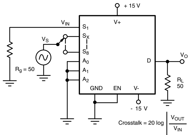
Fig. 6 - Crosstalk
