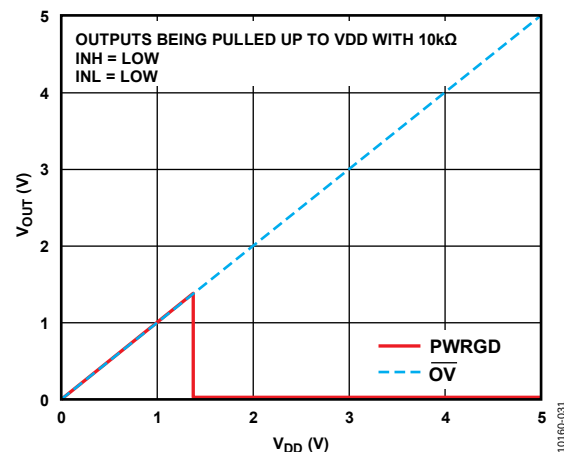
Figure 31. Output Voltage vs. Supply Voltage with Both INH and INL Low
